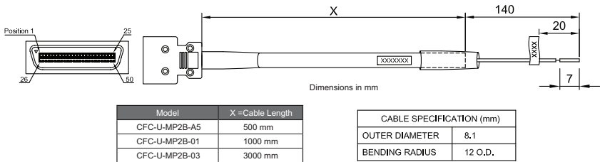
CFC-U-MP2B-xx I/O Pinout for MP2600iec
