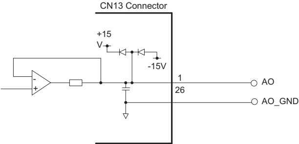
Analog Output Circuit
