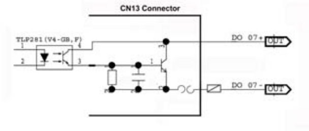
Digital Output Circuit
